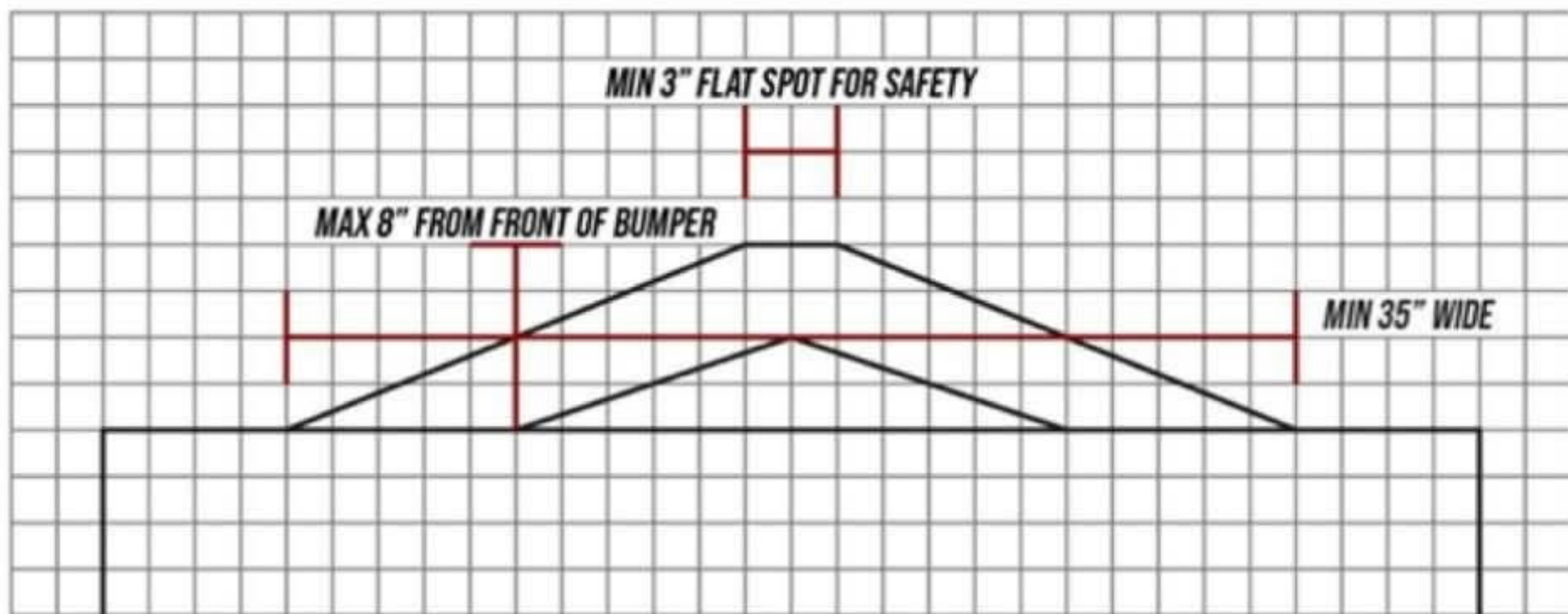
Bumper Diagram
